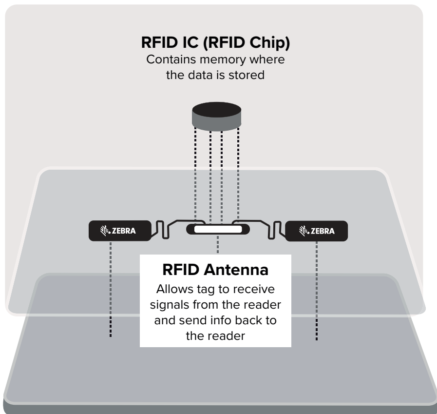
RFID Tag Label or non-adhesive tag with inlay
